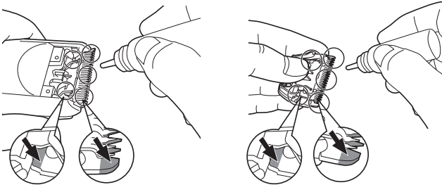
Lubricating using the sliding plate for maintenance
